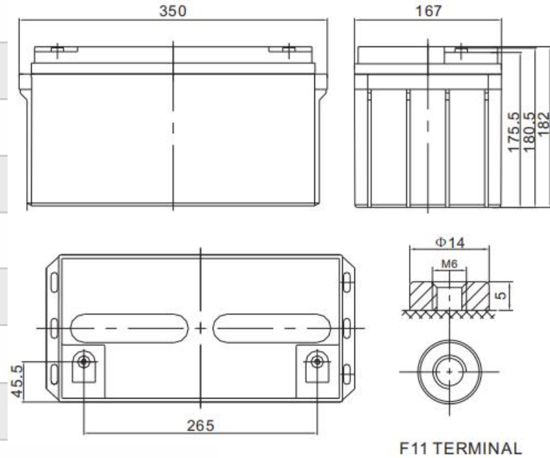
GW12-240W Dimension
